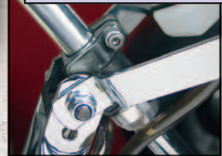
ARROW'S UNIQUE STEERING BUSH WITH CLAMP FOR SIMPLE FRONT END ALIGNMENT
